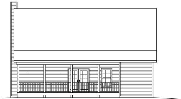
REAR ELEVATION
